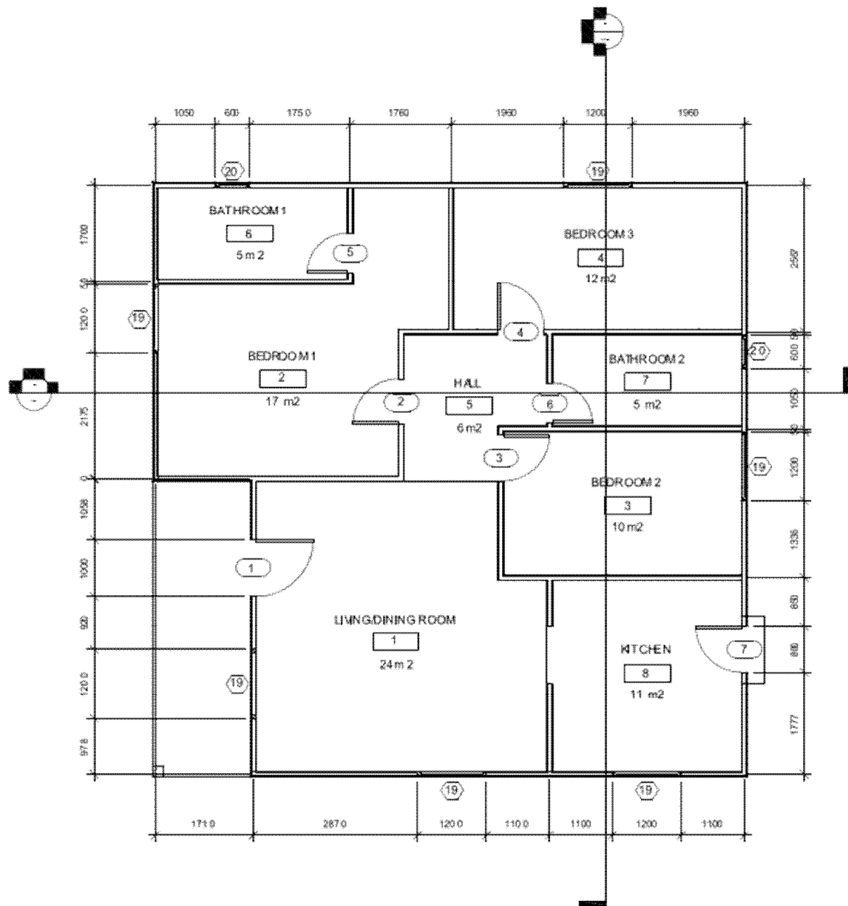
2 Ground Floor Level 1 : 50
